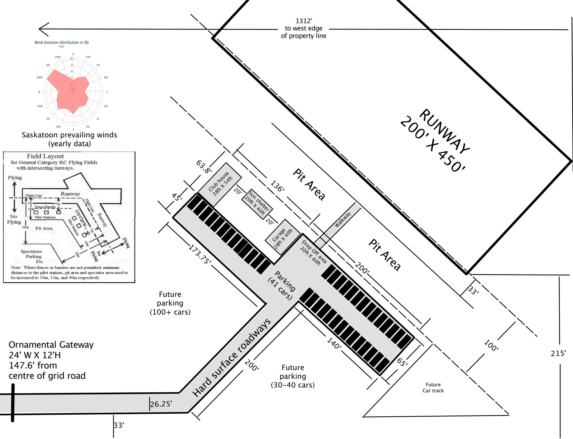
HCRCC proposed field layout B (rev2)
